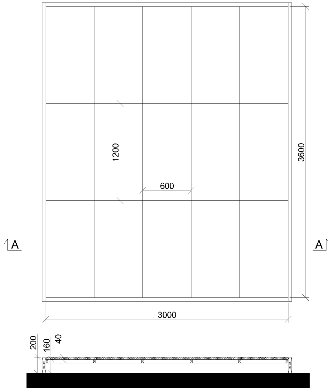
Ewona Excellence H 40 mm, Type E200 mounting Section A-A
