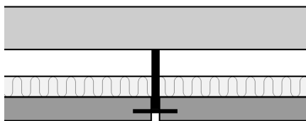
Acoustic plasterboard
